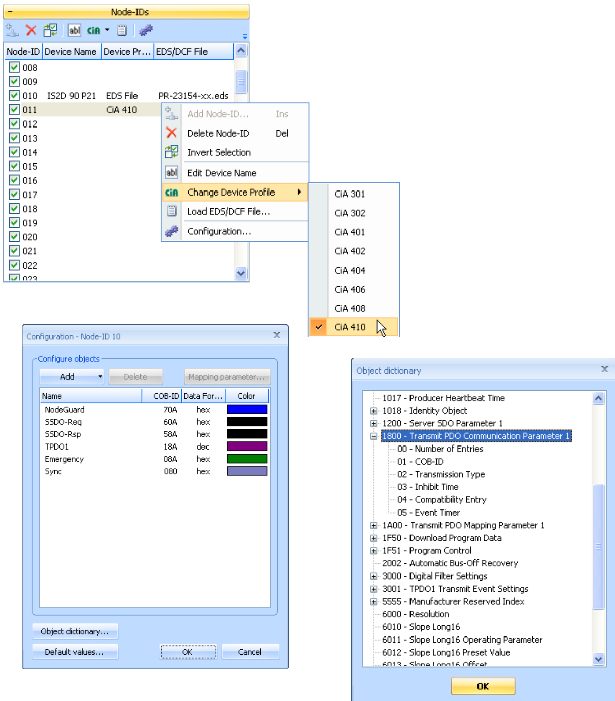
Figure 24: Node configuration (Node IDs)
