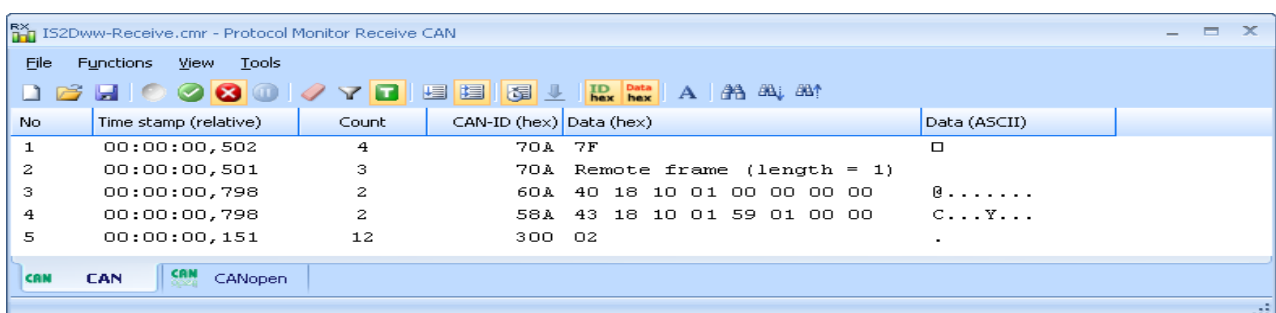
Figure 22: Protocol Monitor Receive: CAN “Overwrite” mode
