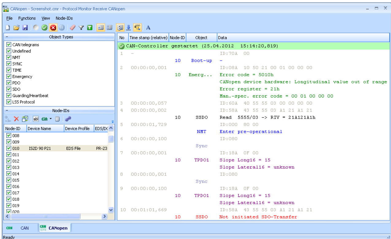
Figure 23: Protocol Monitor Receive: CANopen
