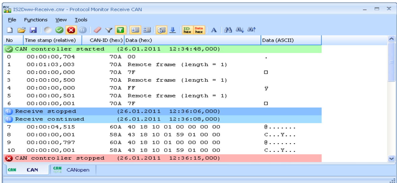
Figure 21: Protocol Monitor Receive: CAN “Scroll” mode
