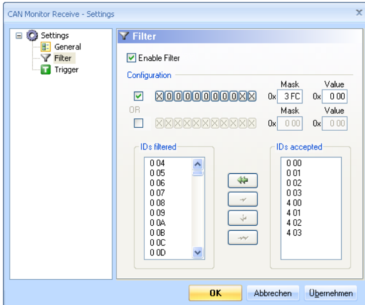
Figure 19: Protocol Monitor Receive: Filter options
