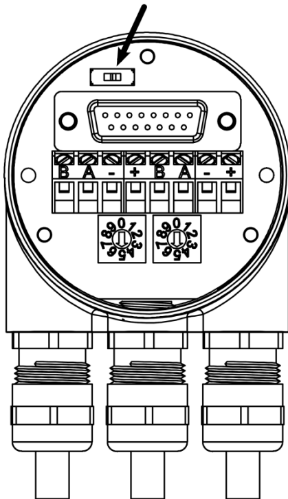
Termination Resistor
